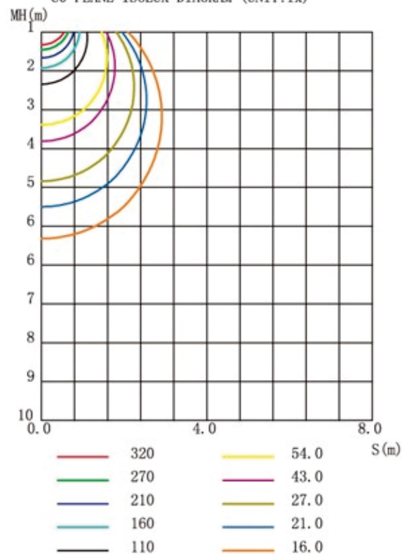
CO PLANE ISOLUX DIAGRAM (UNIT:1x)
